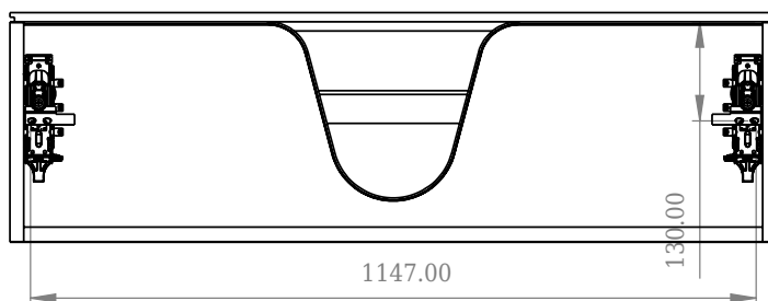
Back View
